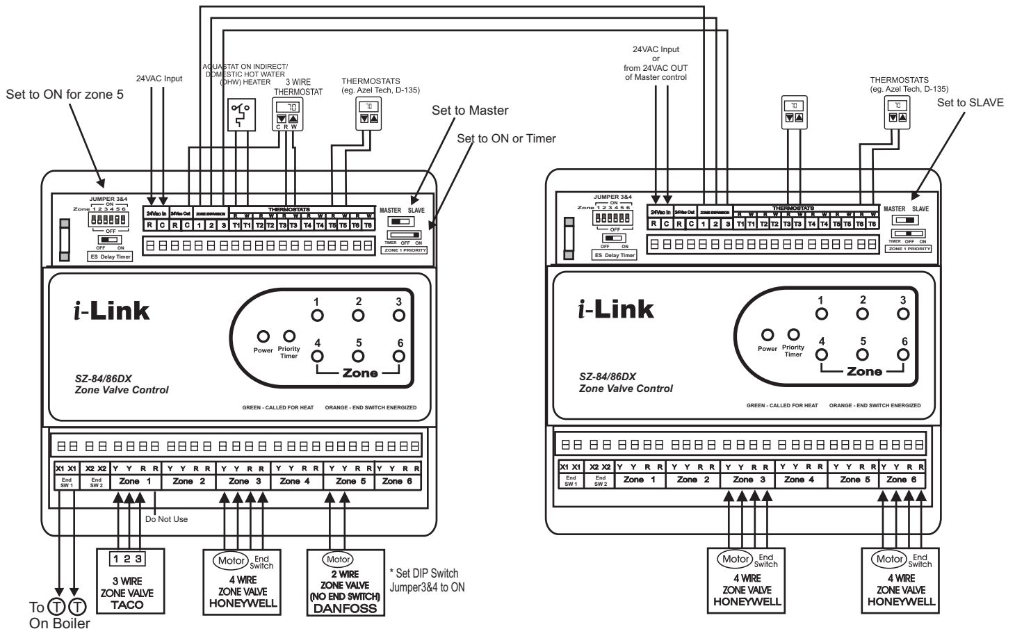
Domestic Hot Water Priority with zone expansion by adding 30061
